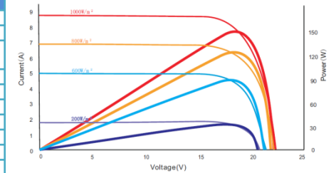
Current-Voltage & Power-Voltage Curve (150-12)
